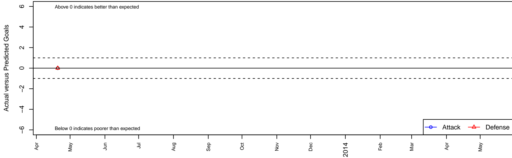
Vancouver Timbers Red B99 Dots are actual minus expected GF (blue circles) and GA (red triangles). Blue line is smoothed change in attack strength. Red is smoothed change in defense strength.
